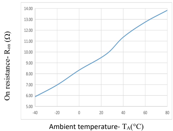
Fig.2 On resistance vs. Ambient temperature characteristics
