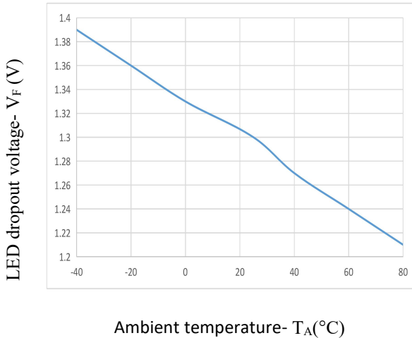
Fig.7 LED dropout voltage vs. Ambient temperature characteristics
